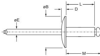
AD ■ ABS LF Large flange Tête large / Flachrundkopf, extragroß / Testa larga / Cabeza ancha
